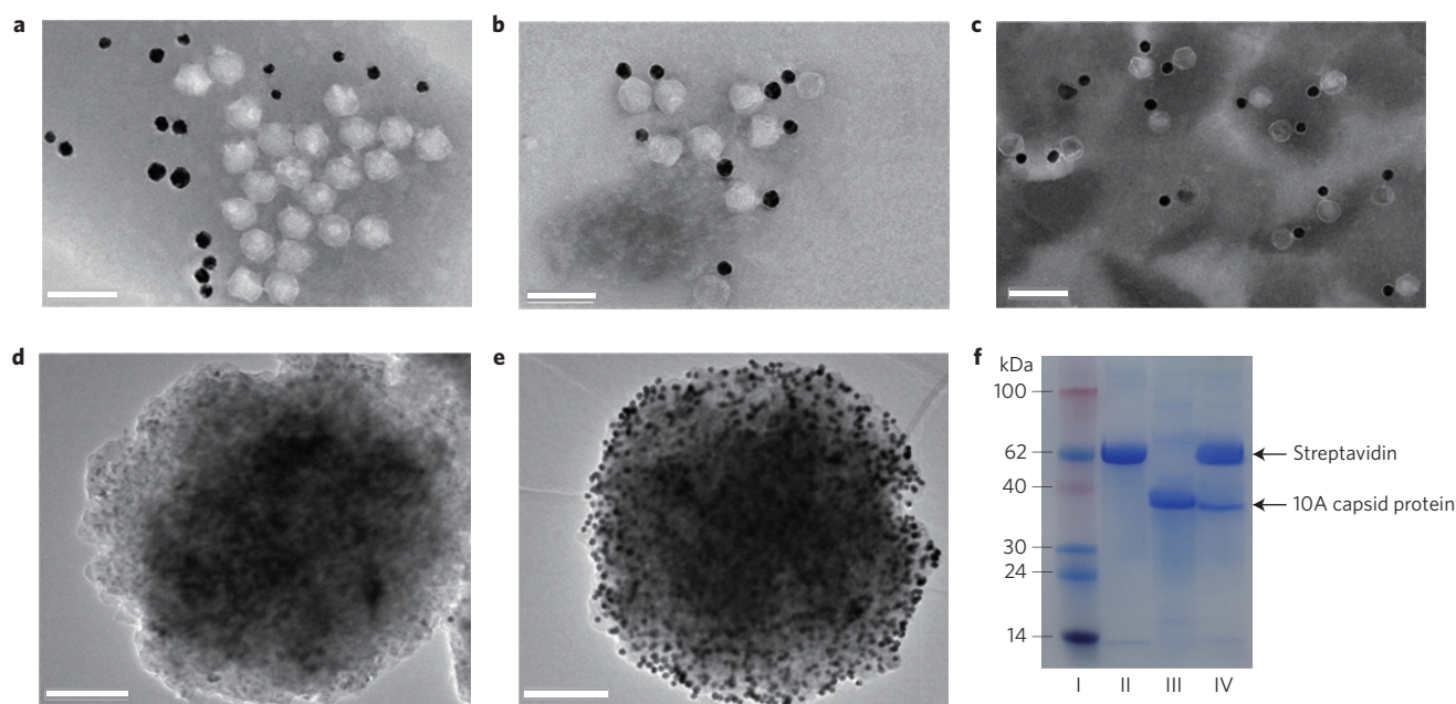
Figure 2 | Preparation and characterization of T7-GNP probes. a , TEM image showing that when T7 phages not displaying GBP were mixed with oligonucleotide-modified GNPs under gentle shaking conditions for 5 h at 25 °C, the T7 phages did not have specific binding interactions with GNPs. b , TEM image of T7-GNP probes showing that when the engineered GNP-binding T7 phages were mixed with oligonucleotide-modified GNPs under the same conditions, T7 phages and GNPs were specifically bound together to form a couple in a one-to-one manner owing to the display of GBP at the tails of T7 phages. c , TEM image of T7-GNP probes stored for up to 12 months. d , TEM image of the MMP generated from a mixture solution containing 40 \mu l of 2-functionalized MMP probes at 2.5 mg ml -1 , 40 \mu l of 1-functionalized GNPs at 2.5 nM and 20 \mu l of an assay buffer for 30 min, followed by washing six times with magnetic separation. e , TEM image of the MMP-GNP complex magnetically separated from a hybridization mixture containing 40 \mu l of 2-functionalized MMP probes at 2.5 mg ml -1 , 40 \mu l of 1-functionalized GNPs at 2.5 nM and 20 \mu l of let-7a at 1 \mu M. The data show that the MMP probe has good ability to hybridize with target miRNA. f , SDS-PAGE analysis of different samples. I, protein marker. II, MMP probes. III, engineered T7 phages. IV, MMP probes separated by a magnetic separator in the presence of target miRNA molecules. These results confirmed the presence of T7 phage in the sandwich complexes. Scale bars, 100 nm ( a-c ); 200 nm ( d,e ).
